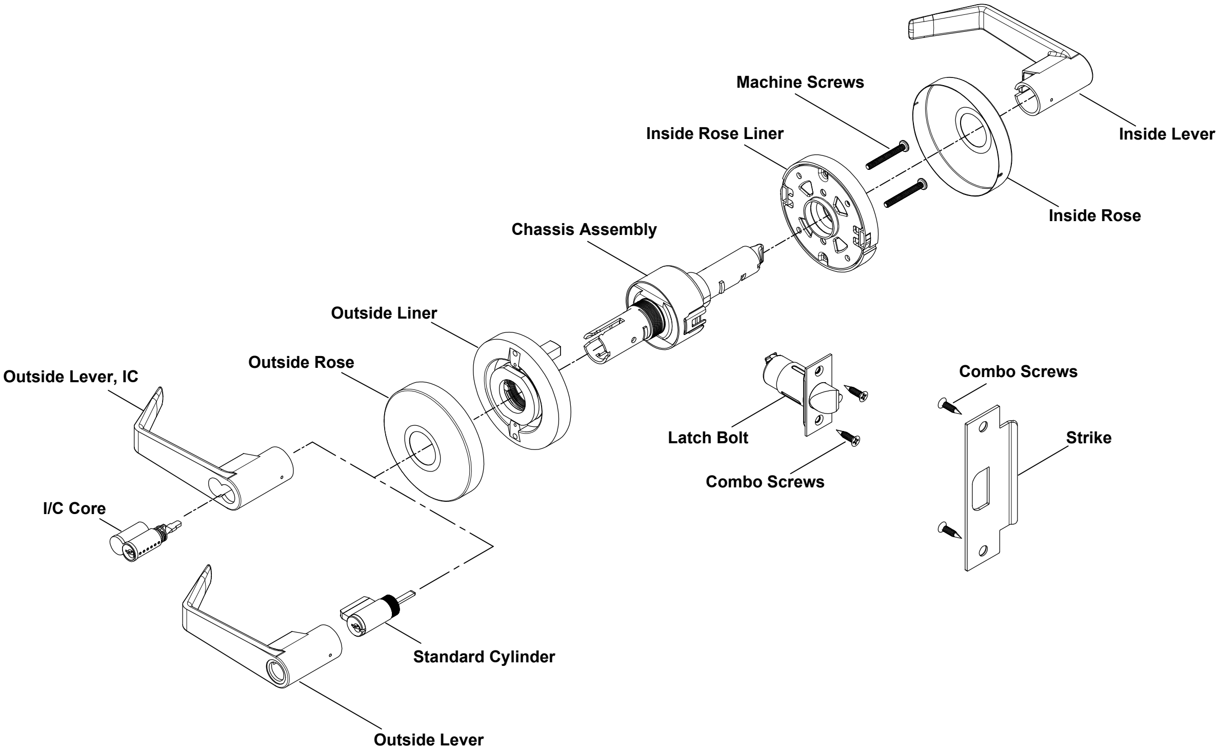
"C500 SERIES" Cylindrical Lock
