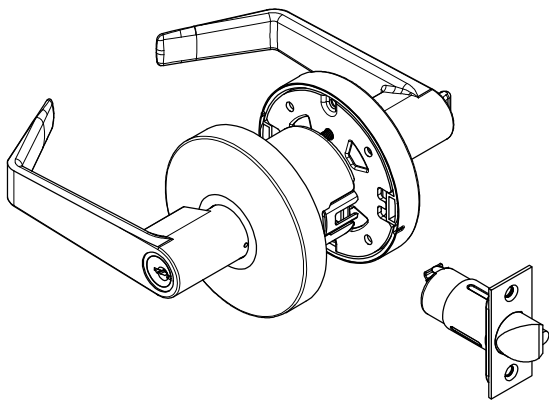
"C500 SERIES" Cylindrical Lock
